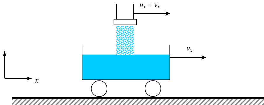
Figure 2. Sketch of the horizontal motion of an open-topped freight car that is filled of water, from a pipe with the same horizontal velocity as the car.
