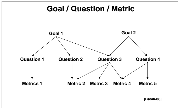
Figure 3: Goal/Question/Metric Paradigm
